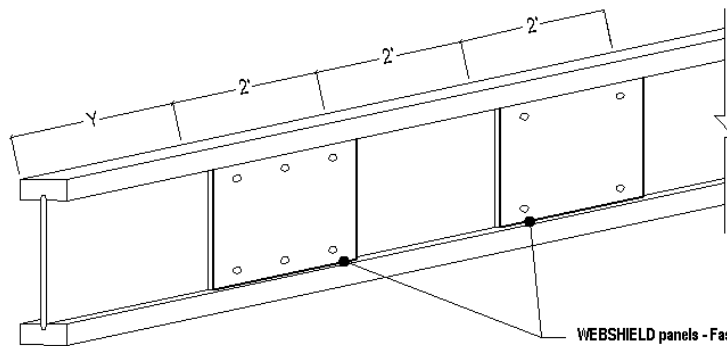
WEBSHIELD panels - Fastening option A and B
