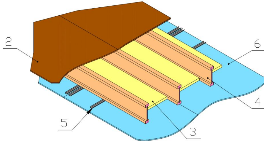
FIGURE 4 – 1-Hour Fire-Rated Floor-Ceiling or Roof-Ceiling Assembly, Design No. 60-02
